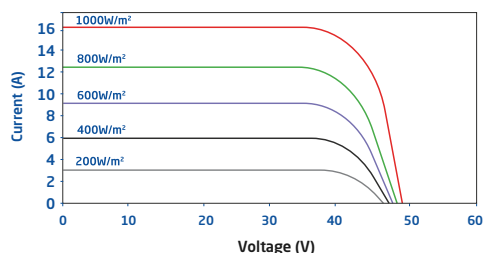
Current-Voltage Curves (ISHTG12R66H650)
